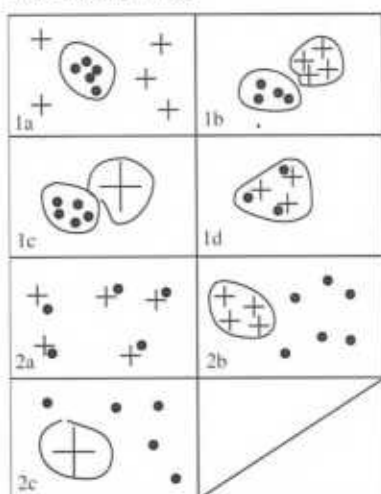
Model Renfrew 1983
