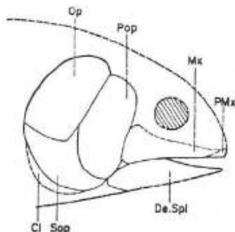
Fig. 80- Colobodus sp. (original de BELTAN, 1972) Alcover / Mont-Rai
