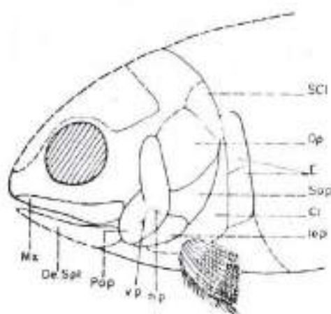
Fig. 84- Parasemionotus villaltai (original de BELTAN, 1972)
